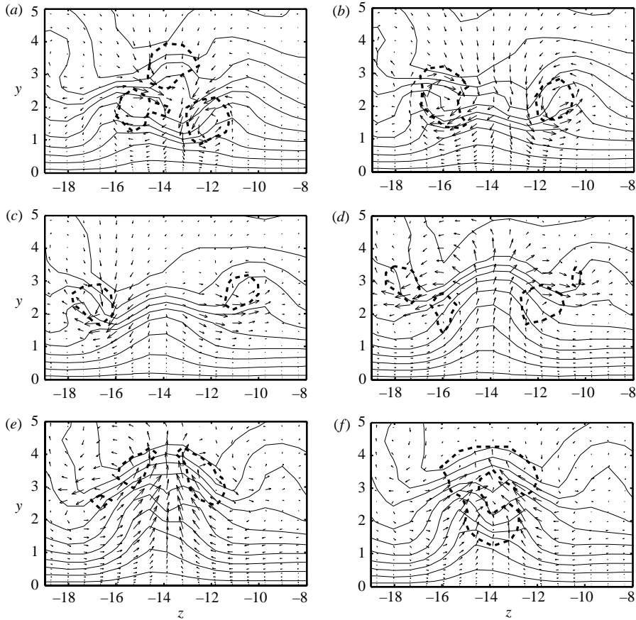
FIGURE 14. Vertical planes in the cross-stream directions showing details of the incipient spots depicted in figure 13. The arrows represent the spanwise and wall-normal velocities, while solid lines indicate constant streamwise velocity from 0.05 to 0.95 with spacing of 0.1. The thick dashed lines represent constant negative values of \lambda_2 and show the core of the vortical structures. (a) x = 350 , (b) x = 352 , (c) x = 354 , (d) x = 357 , (e) x = 359 , (f) x = 361 .
