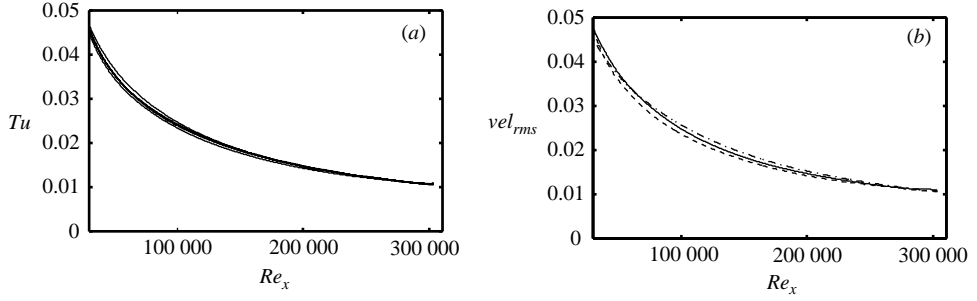
FIGURE 1. (a) Turbulence intensity versus the Reynolds number at 5 different heights above the boundary layer ( y/\delta_0^* = 30, 40, 50, 60, 70 ; L = 5\delta_0^* ). (b) Root mean square values of the three velocity components versus the Reynolds number for L = 5\delta_0^* and y/\delta_0^* = 40 . —, u_{rms} ; ---, v_{rms} ; ···, w_{rms} .
